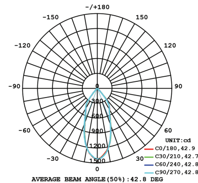
15W 1-LIGHT GIMBAL WIDE CLEAR
